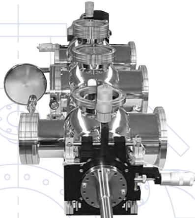
Multi-chamber custom research and development system consisting of three chambers and a variety of sample transfer and manipulation devices
